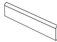
Rodapié Canto Romo Skirting bullnose 8 x 60 cm (3,2" x 24")
